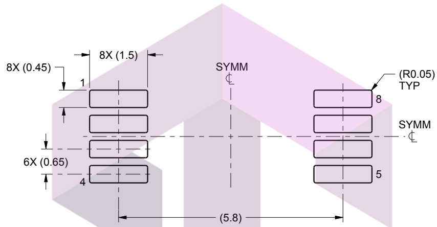
LAND PATTERN EXAMPLE SCALE:10X
