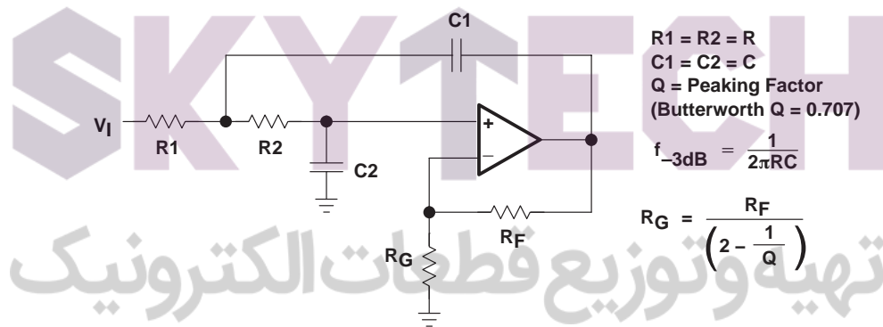
Figure 61. 2-Pole Low-Pass Sallen-Key Filter
